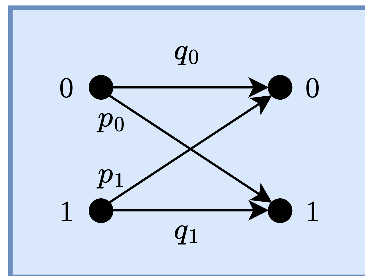
Combined model (BAC-ZC)
