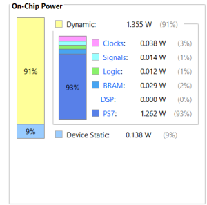
(b) Power summary sau implementation.
