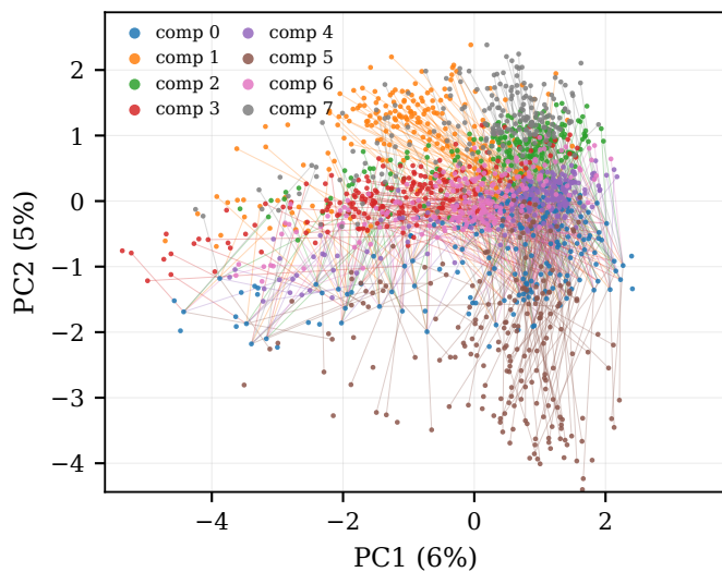
Default init (no alignment pressure) \cos = 0.132 twin dist = 1.37 \times cloud radius
