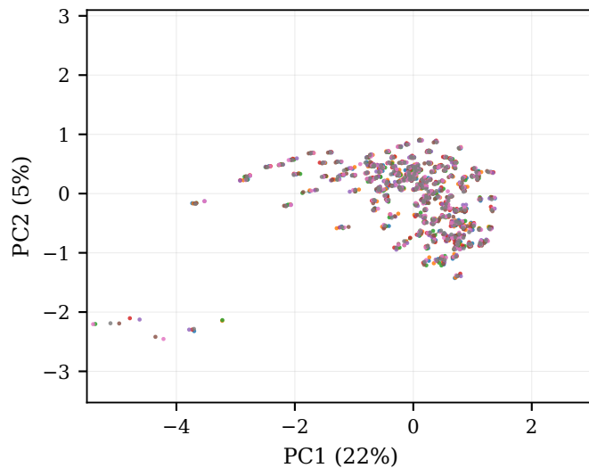
Init-copy (embeddings + head shared at init) \cos = 0.981 twin dist = 0.20 \times cloud radius
