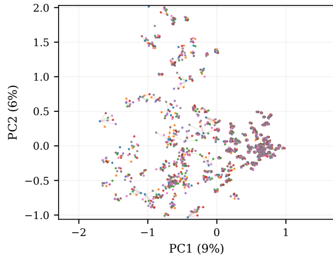
InfoNCE (explicit layer-4 alignment) \cos = 0.963 twin dist = 0.25 \times cloud radius
