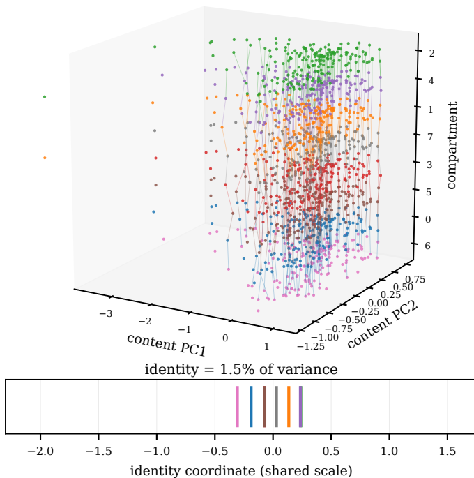
Init-copy (embeddings + head shared at init) cos 0.981 \rightarrow 0.996 with identity removed
