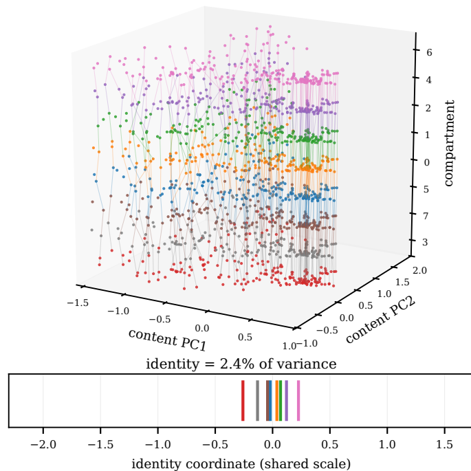
InfoNCE (explicit layer-4 alignment) cos 0.963 \rightarrow 0.984 with identity removed
