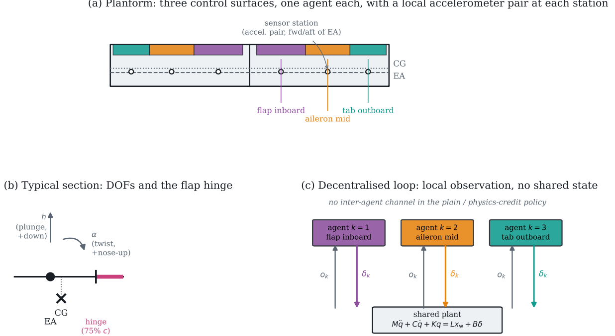
Fig. 1 The testbed. (a) Planform, agent colours matched throughout the paper. (b) The typical-section degrees of freedom and flap hinge. (c) The information structure: each agent closes its own loop through the shared plant, with no inter-agent channel in the plain and physics-credit policies.
