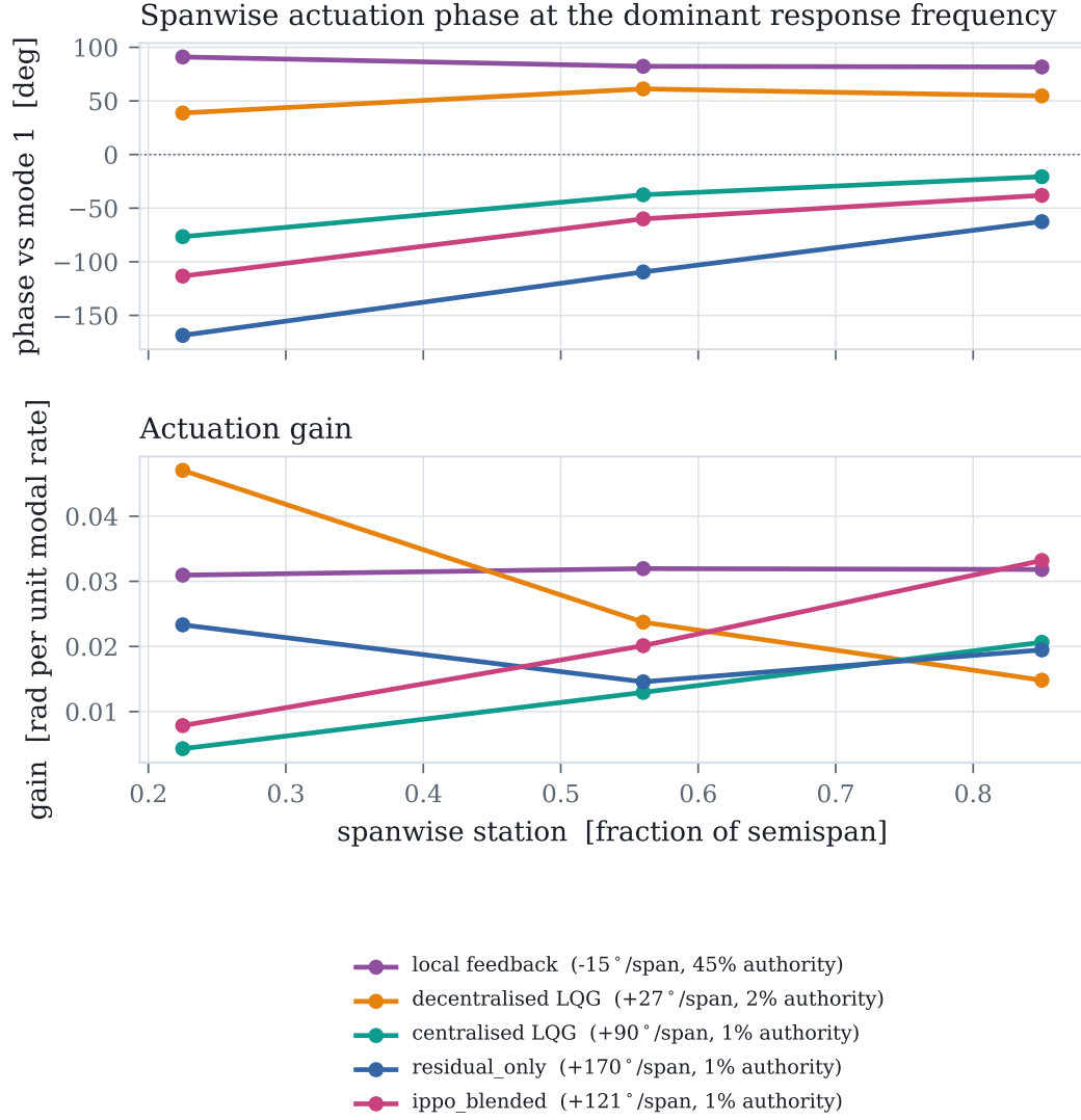
Fig. 2 Spanwise actuation phase (top) and gain (bottom) at each controller's dominant response frequency. A sloped phase profile is a travelling-wave pattern matched to the mode shape; a flat profile is purely local reaction.
