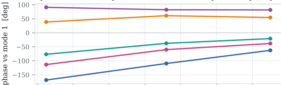
Spanwise actuation phase at the dominant response frequency
