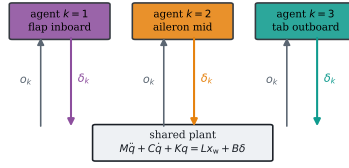
(c) Decentralised loop: local observation, no shared state no inter-agent channel in the plain / physics-credit policy
