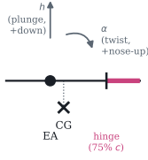
Figure 1: The testbed. (a) Planform, agent colours matched throughout the paper. (b) The typical-section degrees of freedom and flap hinge. (c) The information structure: each agent closes its own loop through the shared plant, with no inter-agent channel in the plain and physics-credit policies.
