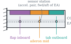
(a) Planform: three control surfaces, one agent each, with a local accelerometer pair at each station
