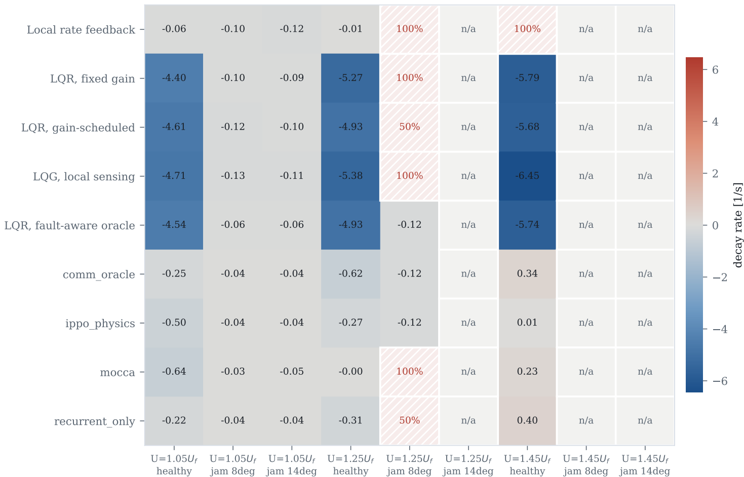
Energy decay rate [1/s] by controller and flight condition negative = suppressed; hatched = diverged; n/a = infeasible for any controller
