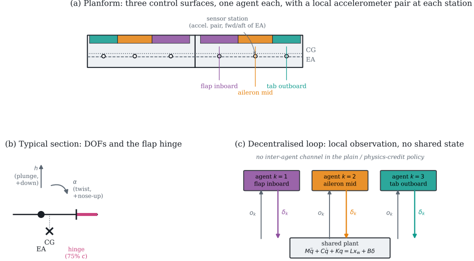
Figure 1: The testbed. (a) Planform, agent colours matched throughout the paper. (b) The typical-section degrees of freedom and flap hinge. (c) The information structure: each agent closes its own loop through the shared plant, with no inter-agent channel in the plain and physics-credit policies.
