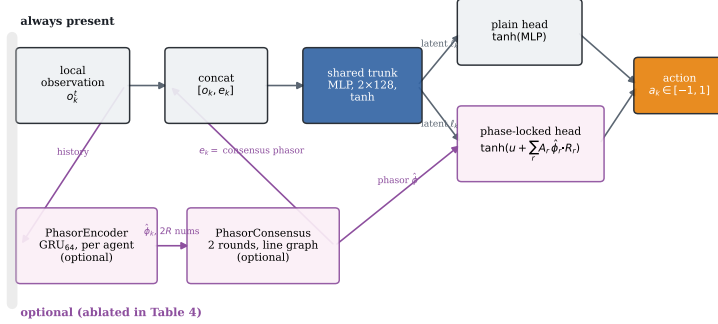
Figure 3: The policy network. Grey boxes and the plain head are present in every variant; the pink boxes and the phase-locked head are the mechanisms ablated in Table 4, so recurrent_only keeps the encoder but not consensus or the head, mocca_nohead keeps the encoder and consensus but ends in the plain head, and mocca is the full diagram.
