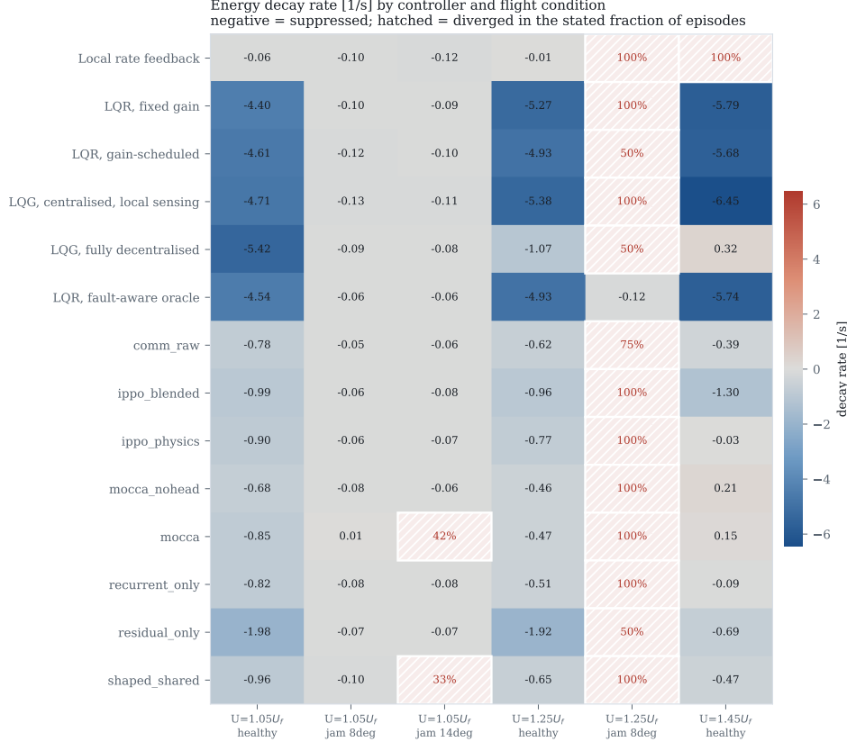
Figure 5: Decay rate by controller and condition. Hatching marks divergence.
