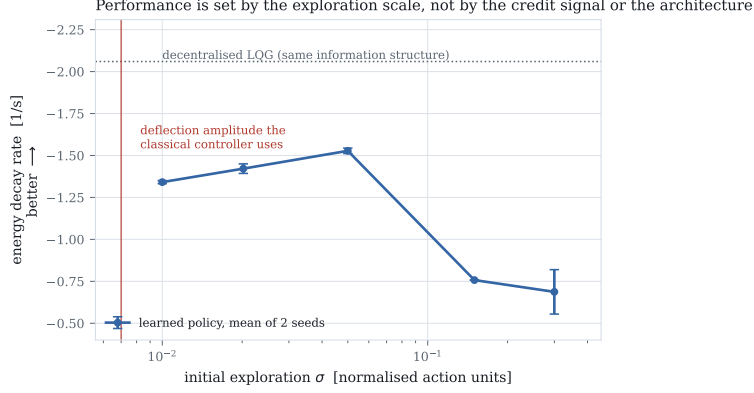
Figure 8: Decay rate against initial exploration standard deviation, all else fixed. The vertical line marks the deflection amplitude the classical controller uses. Two seeds per point.
