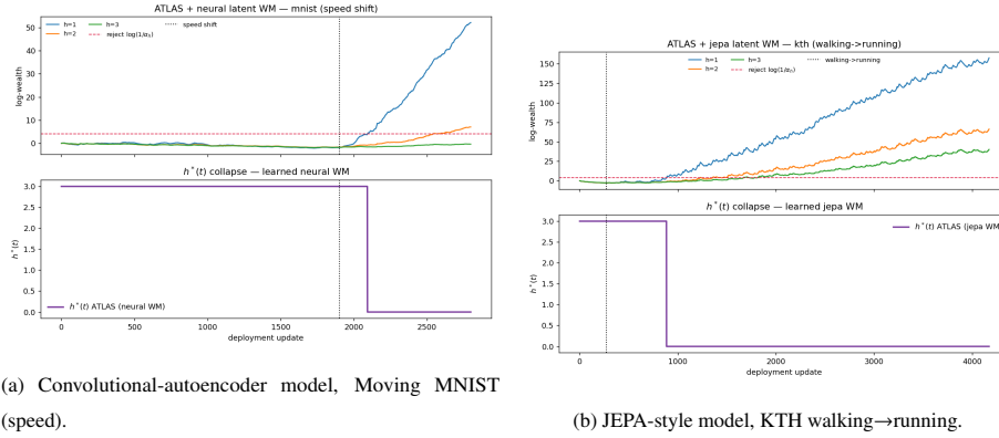
Figure 6: ATLAS monitoring learned neural world models: a valid in-distribution null (flat wealth) followed by h^*(t) collapse at the shift, for both a convolutional autoencoder and a JEPA-style model.
