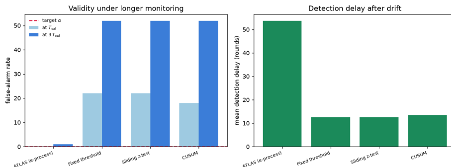
Figure 9: ATLAS versus competitor monitors. Left: false-alarm rate at the calibration horizon and at a 3\times longer horizon—only ATLAS stays below \alpha (dashed) as monitoring continues; the tuned baselines inflate. Right: mean detection delay. The baselines’ shorter delay is a direct consequence of the looser (invalid) alarm behavior seen on the left.
