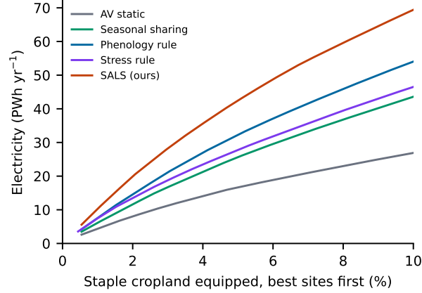
Figure 8: Supply curve under the baseline climate: cumulative electricity when sites are equipped in order of decreasing electricity per hectare, against the share of staple cropland (physical area) equipped. Each controller is evaluated at the density that keeps its mean retention at 0.9.
