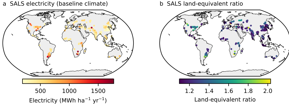
Figure 9: SALS electricity (a) and land-equivalent ratio (b) at the pooled held-out sites (baseline climate, mean of seasons 2015–2019).
