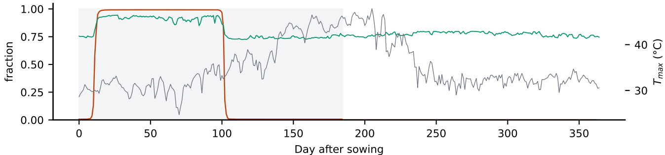
wheat (rainfed), India (22.5, 79.5), GCR 0.200, +3 °C, season sown 2016
