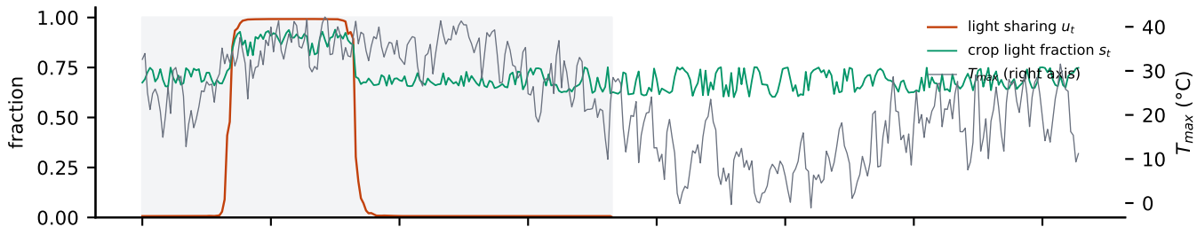
wheat (rainfed), India (22.5, 79.5), GCR 0.200, +3 °C, season sown 2016
