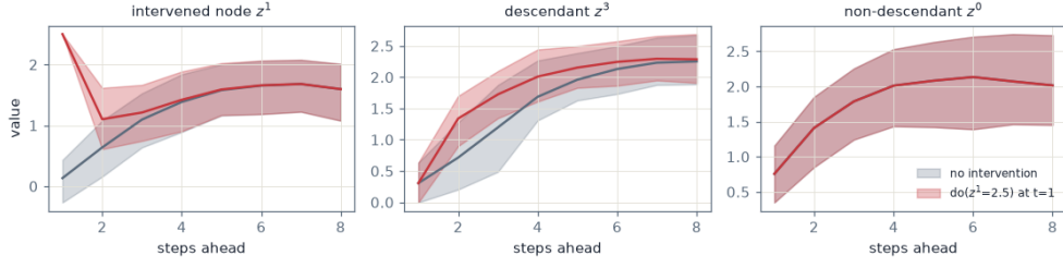
Fig. 2 Graph surgery in imagination on the ground-truth benchmark of Section 4. The query \text{do}(z^1=2.5) pins the intervened variable at the surgery step (left), shifts the distribution of its descendant (middle), and leaves the non-descendant’s imagined future exactly unchanged—the intervention band coincides with the no-intervention band (right). A monolithic model cannot make this promise.
