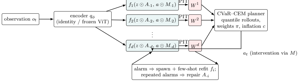
Fig. 4 CAIRN architecture. Observations are encoded into a factored latent state; each variable’s mechanism sees only its masked parents and action targets and outputs quantiles. Each mechanism’s PIT residuals feed its own betting wealth W^i , which weights the mechanism library, inflates rollout uncertainty, and—upon anytime-valid alarms—triggers localized refits and structure repair. The planner acts through quantile rollouts and thus routes around unhealthy mechanisms.
