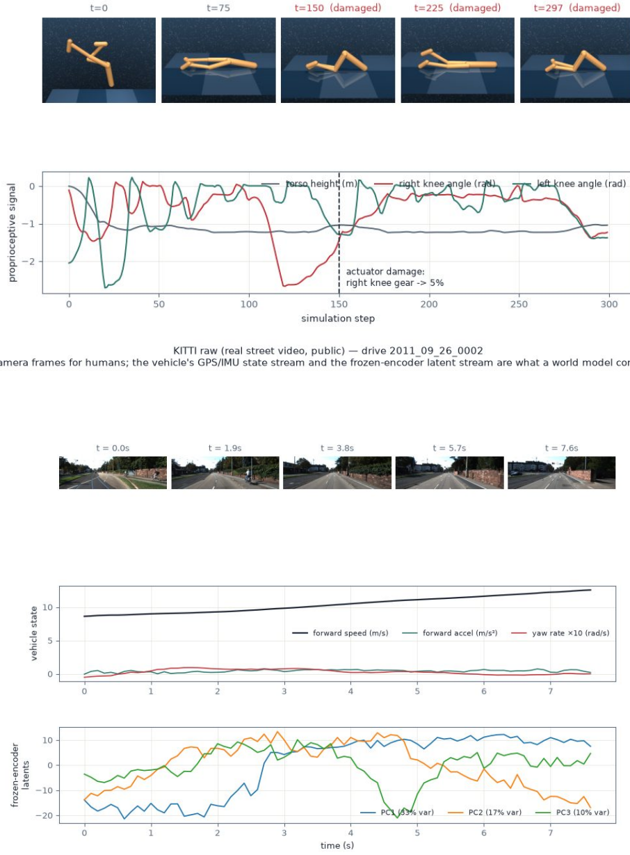
Fig. 8 The road to physical instantiations, illustrated with real data processed by our pipeline. Top: a DeepMind Control walker episode in which the right-knee actuator silently loses 95% of its torque at the dashed line; one proprioceptive trace collapses while the others keep their range—a one-mechanism shift in the wild, and exactly the signature the e-gates localize. Bottom: real street video (KITTI) processed by the frozen-encoder pathway of Section 3.1: camera frames, the vehicle’s measured state stream, and the first three principal components of frozen DINOv2 features per frame—a smooth latent state stream obtained from raw video without any training, over which CAIRN’s mechanisms and gates operate unchanged.
