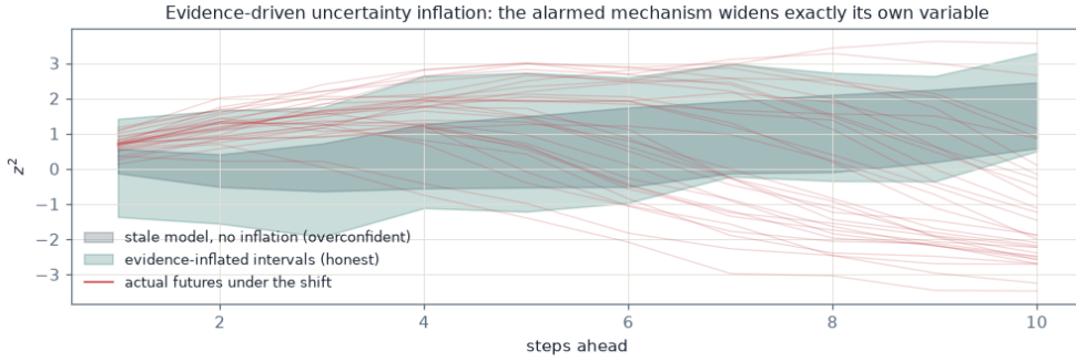
Fig. 7 Evidence-driven uncertainty inflation on the shifted variable. The stale mechanism’s old intervals (grey) miss the actual post-shift futures (thin lines); inflating the spread of exactly the alarmed mechanism (shaded, capped by (10)) restores honest coverage without touching healthy variables.
