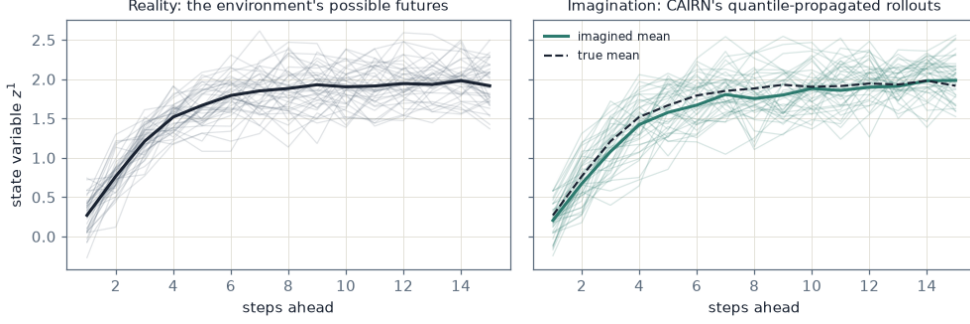
Fig. 1 What a world model does. Left: forty futures that the real environment of Section 4 can produce from one state under one action plan. Right: forty futures CAIRN imagines for the same situation by propagating samples through its per-variable quantile heads. A useful world model must reproduce not only the mean of what will happen (dashed) but the spread of what could.
