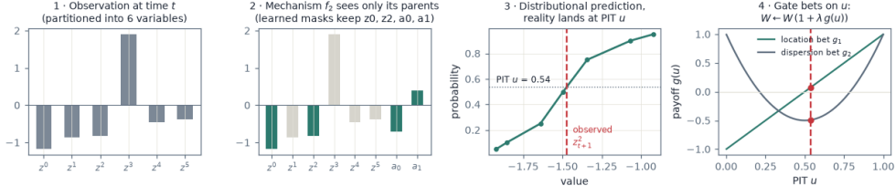
Fig. 3 One transition through CAIRN. (1) The observation is partitioned into variables. (2) Mechanism f_2 receives only the inputs its learned causal masks admit—here two parent variables and both action coordinates; all other inputs are zeroed. (3) The mechanism predicts a full distribution through seven quantiles, and the realized next value lands at PIT u = 0.54 , near the middle, as it should when the mechanism is valid. (4) The gate evaluates its location and dispersion payoffs at u and updates its wealth by (4).
