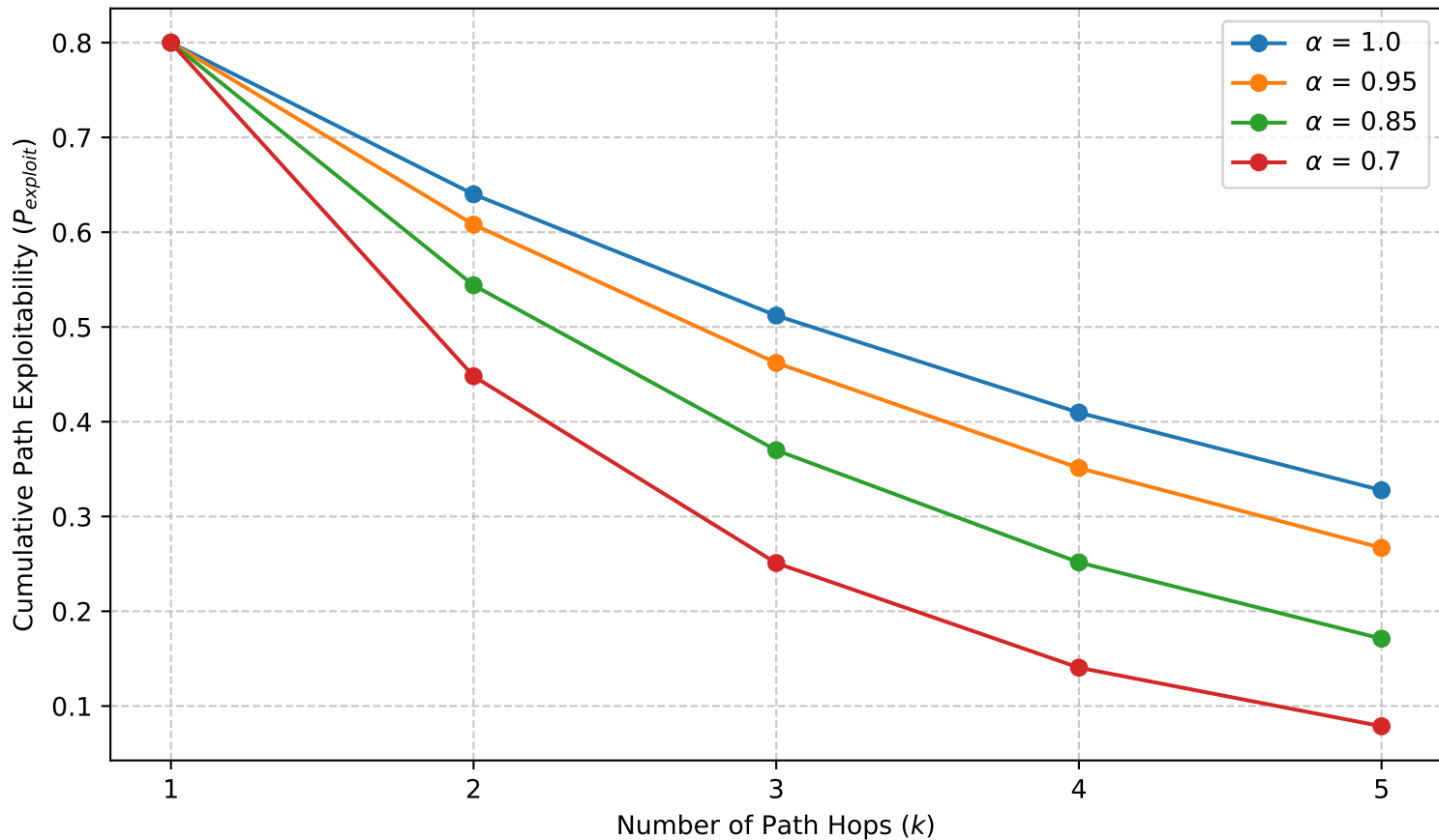
Effect of Chaining Decay Factor over Multi-Hop Attacks
