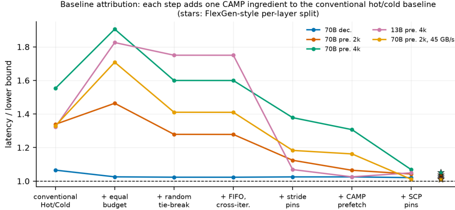
Figure 5: Baseline attribution: latency relative to the lower bound as each ingredient is added to a conventional hot/cold baseline. Stars: the tuned FlexGen-style split.
