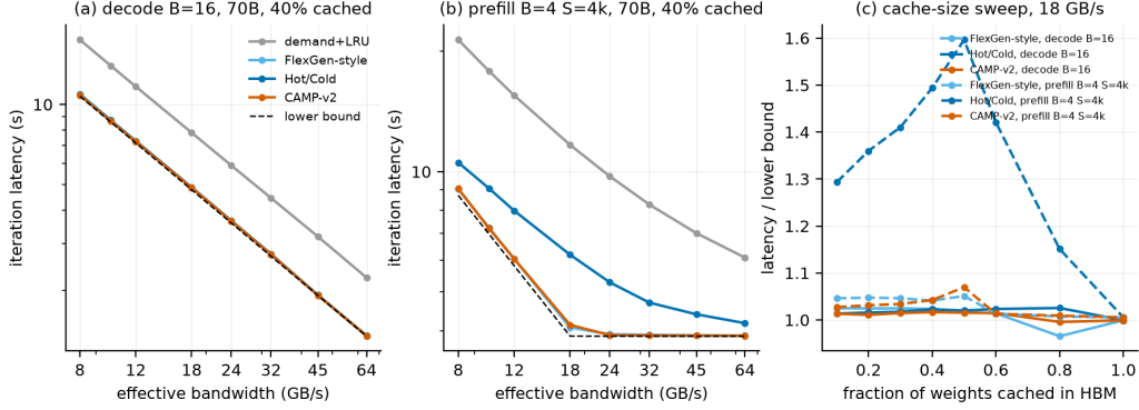
Figure 11: (a, b) Iteration latency versus effective bandwidth for decode and balanced prefill (70B). (c) Latency relative to the lower bound versus the cached fraction of the weights at 18 GB/s.
