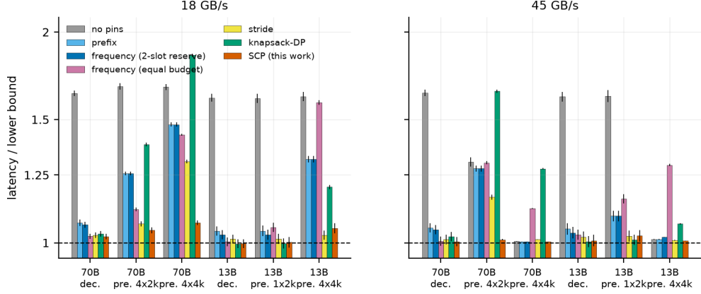
Figure 6: Pin-selection rules with the prefetcher and eviction fixed (latency relative to the lower bound; 10 seeds, 95% confidence bars). Placement matters when compute and transfer are comparable (prefill at 18 GB/s) and not in link-bound decode.
