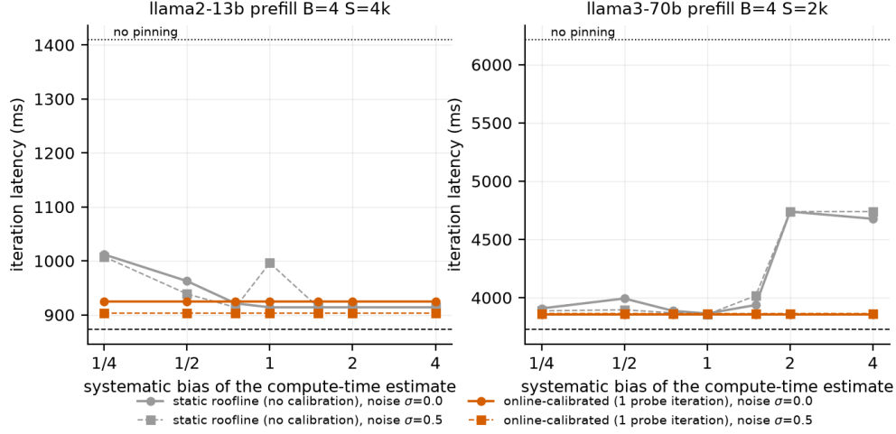
Figure 8: Iteration latency when SCP is planned from a compute estimate with systematic bias (x-axis) and per-layer noise, with and without online calibration. Dotted: no pinning; dashed: lower bound.
