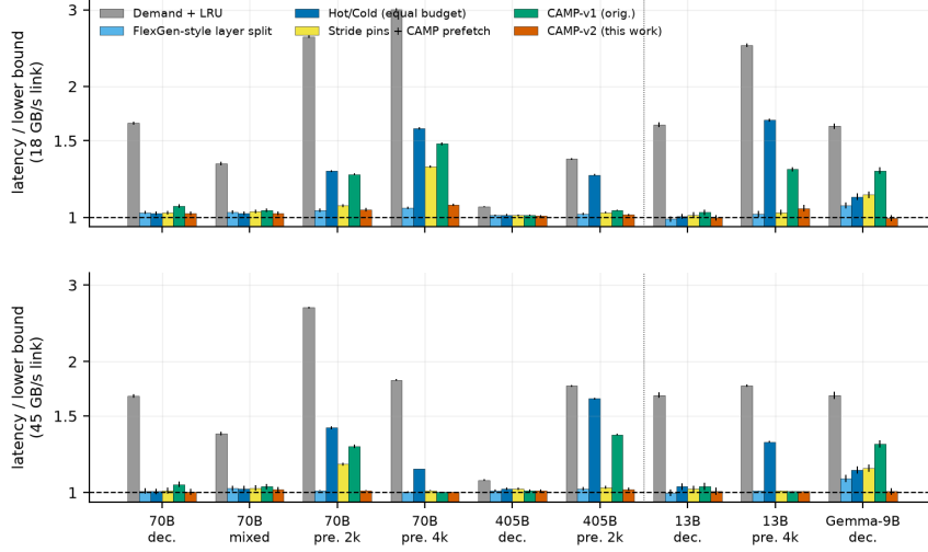
Latency relative to max(compute-only time, link-time lower bound); lower is better. Left of dotted line: 70B/405B; right: 13B/Gemma at 40% cache
