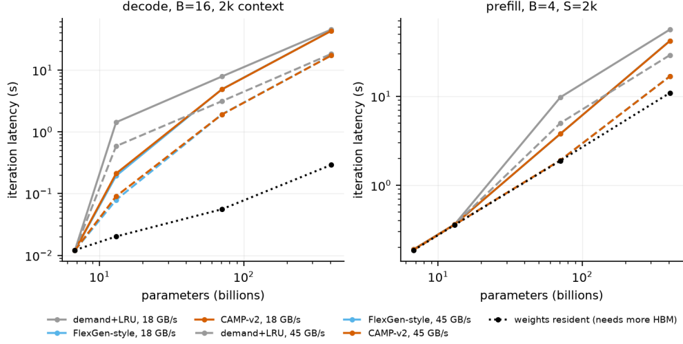
Figure 10: Iteration latency versus model size at fixed 80 GB HBM (B=16 decode with 2k context; B=4, S=2k prefill). The dotted line is the latency if all weights were resident.
