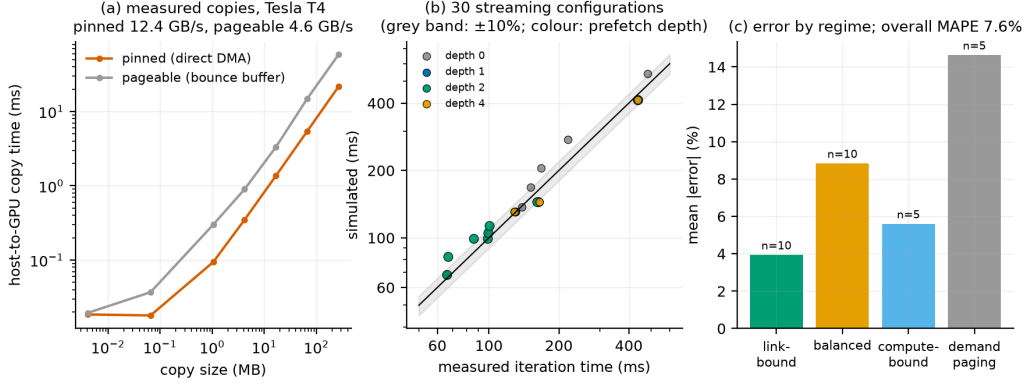
Figure 2: Check on a Tesla T4 (PCIe-attached GPU, pinned host memory as the pool). (a) Measured host-to-GPU copy time versus size for pinned and pageable memory. (b) Simulated versus measured iteration time for the 30 streaming configurations. (c) Mean absolute error by regime; the ratio of compute to copy time per unit defines the regime.
