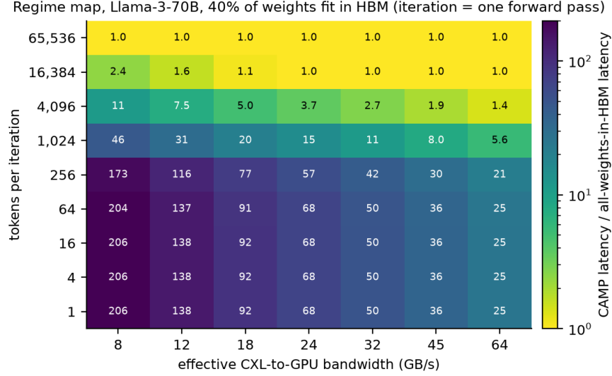
Figure 3: Regime map: CAMP iteration latency relative to all-weights-in-HBM, Llama-3-70B with 40% of the weights cached, as a function of tokens per iteration and effective CXL-to-GPU bandwidth (each cell: four seeds).
