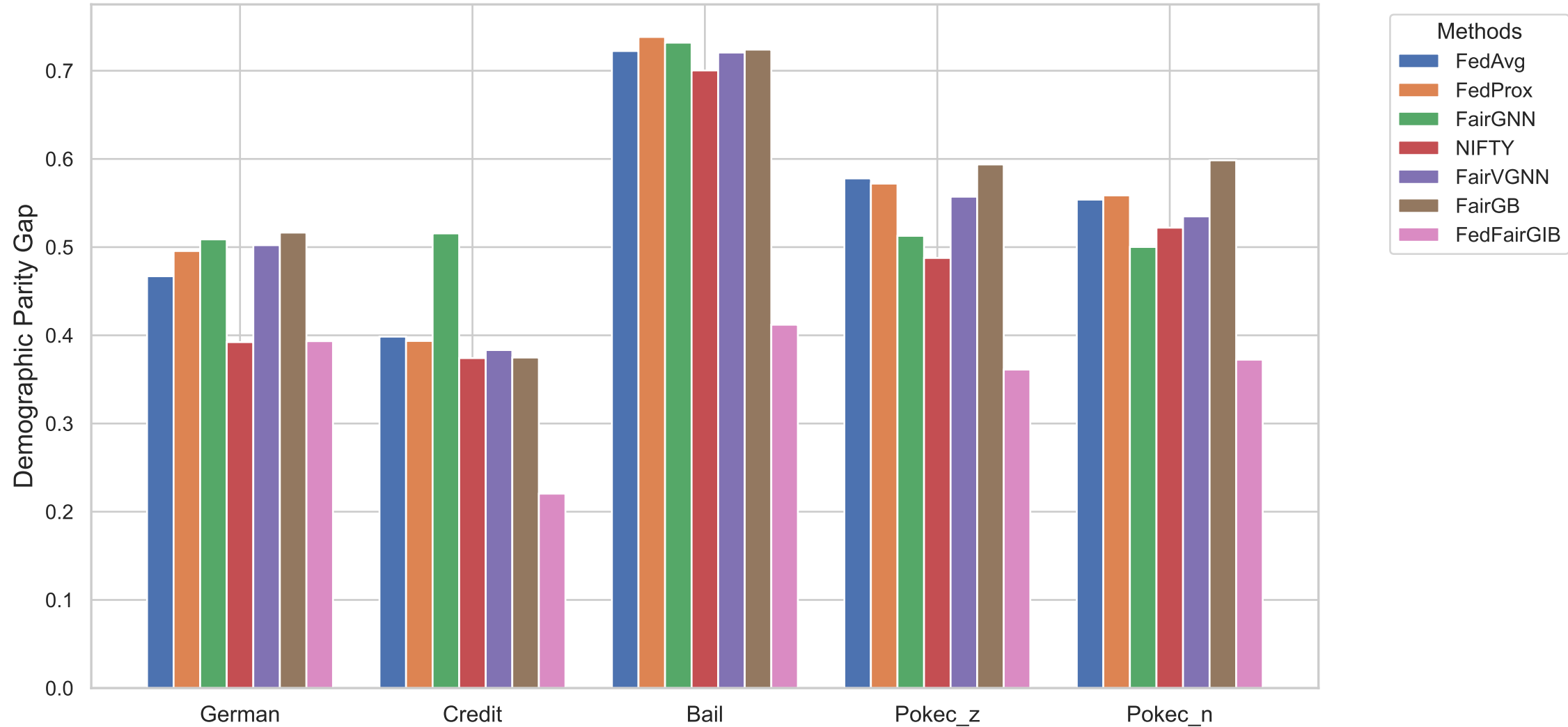
D_DP across Datasets (IID Split)
