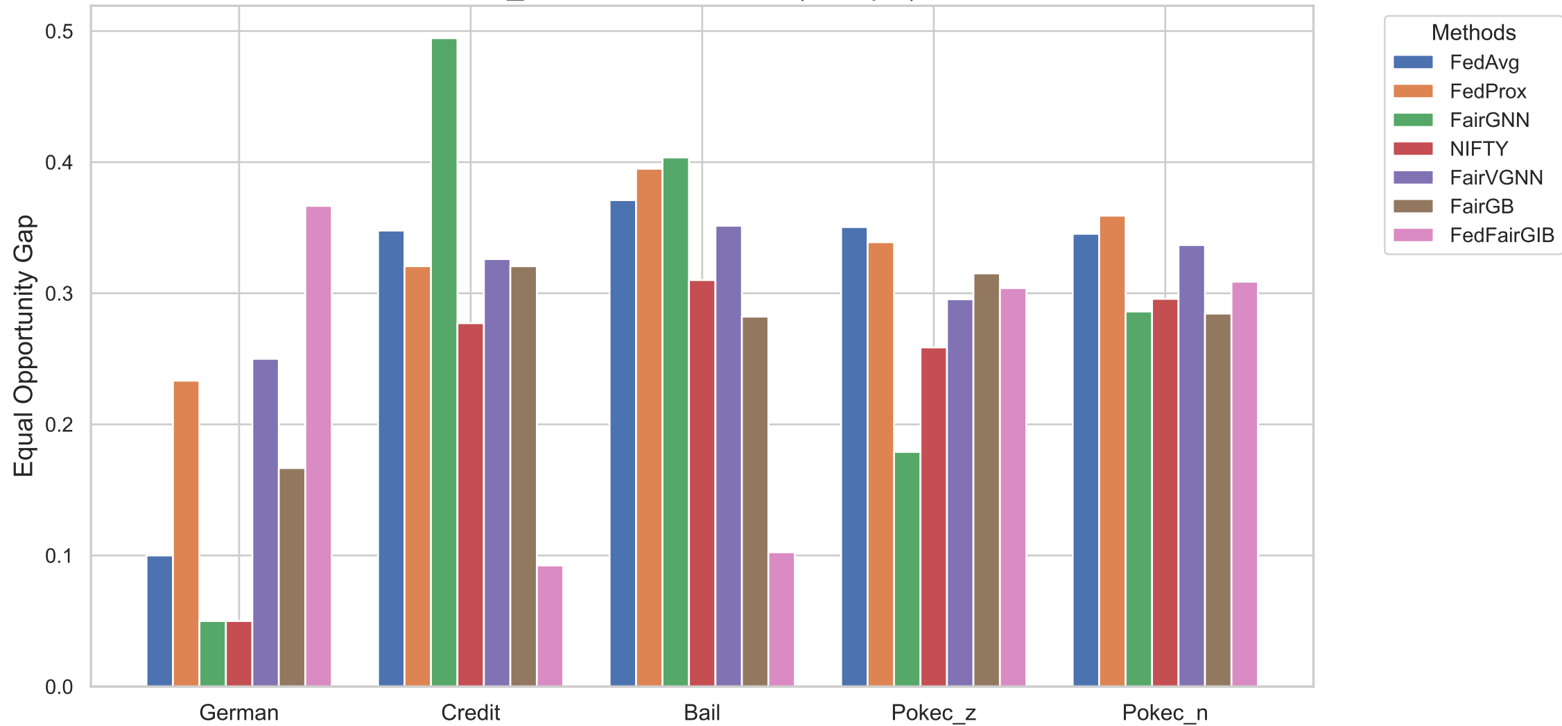
D_EO across Datasets (IID Split)
