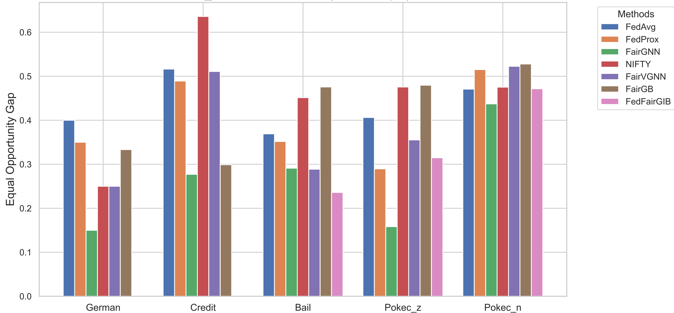
D_EO across Datasets (NONIID Split)
