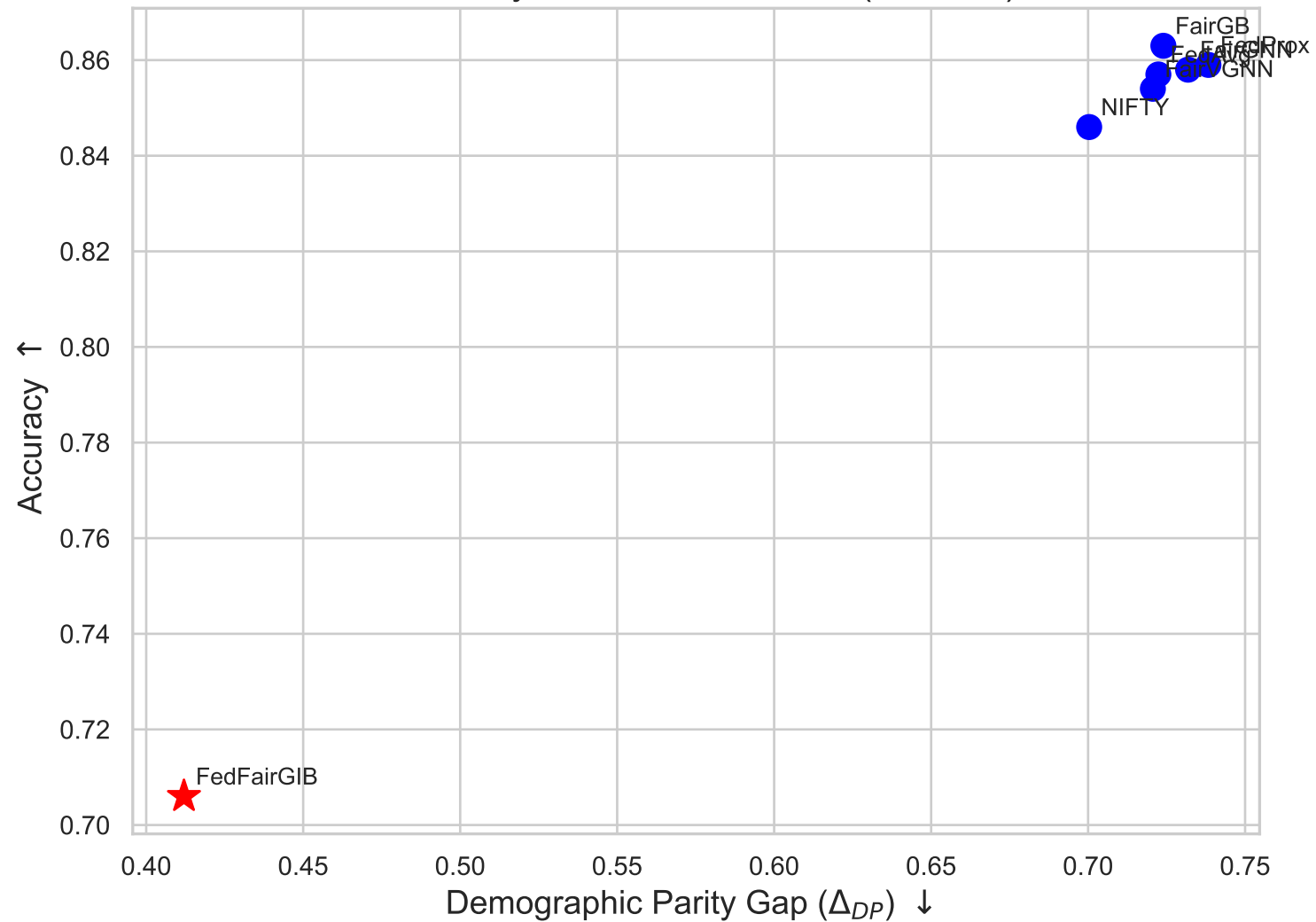
Accuracy-Fairness Trade-off (Bail, IID)
