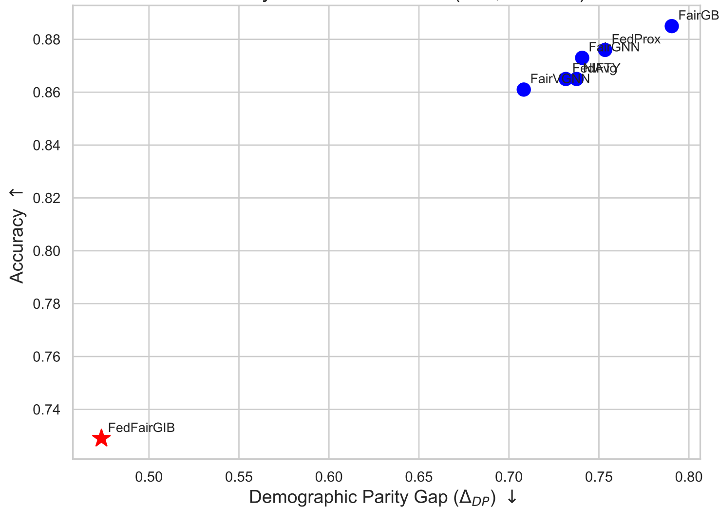
Accuracy-Fairness Trade-off (Bail, NONIID)
