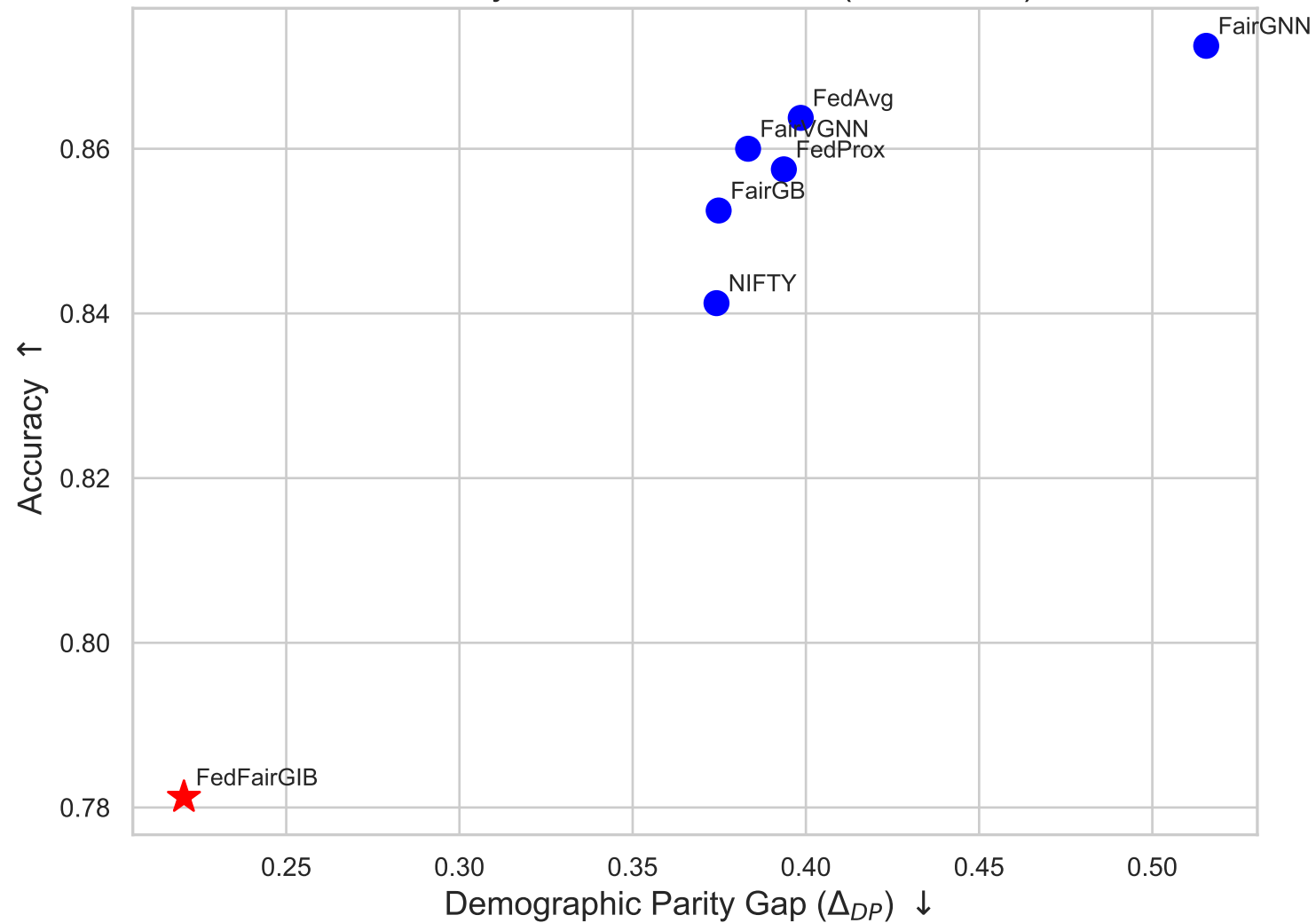
Accuracy-Fairness Trade-off (Credit, IID)
