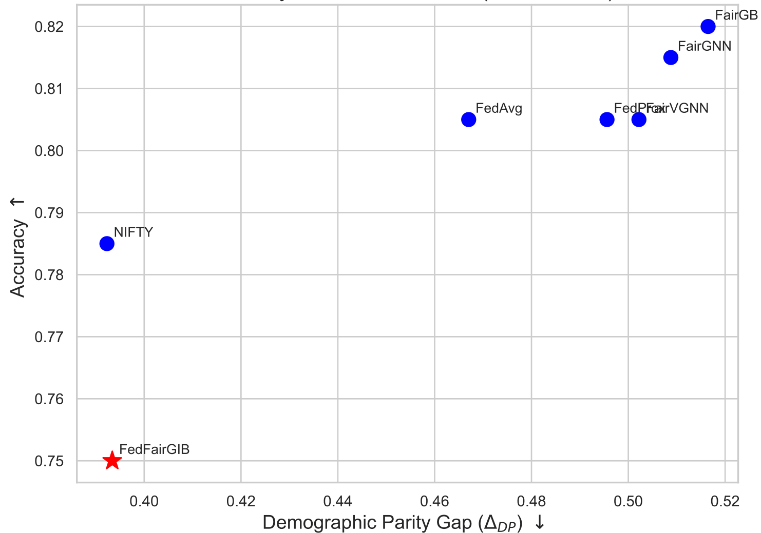
Accuracy-Fairness Trade-off (German, IID)
