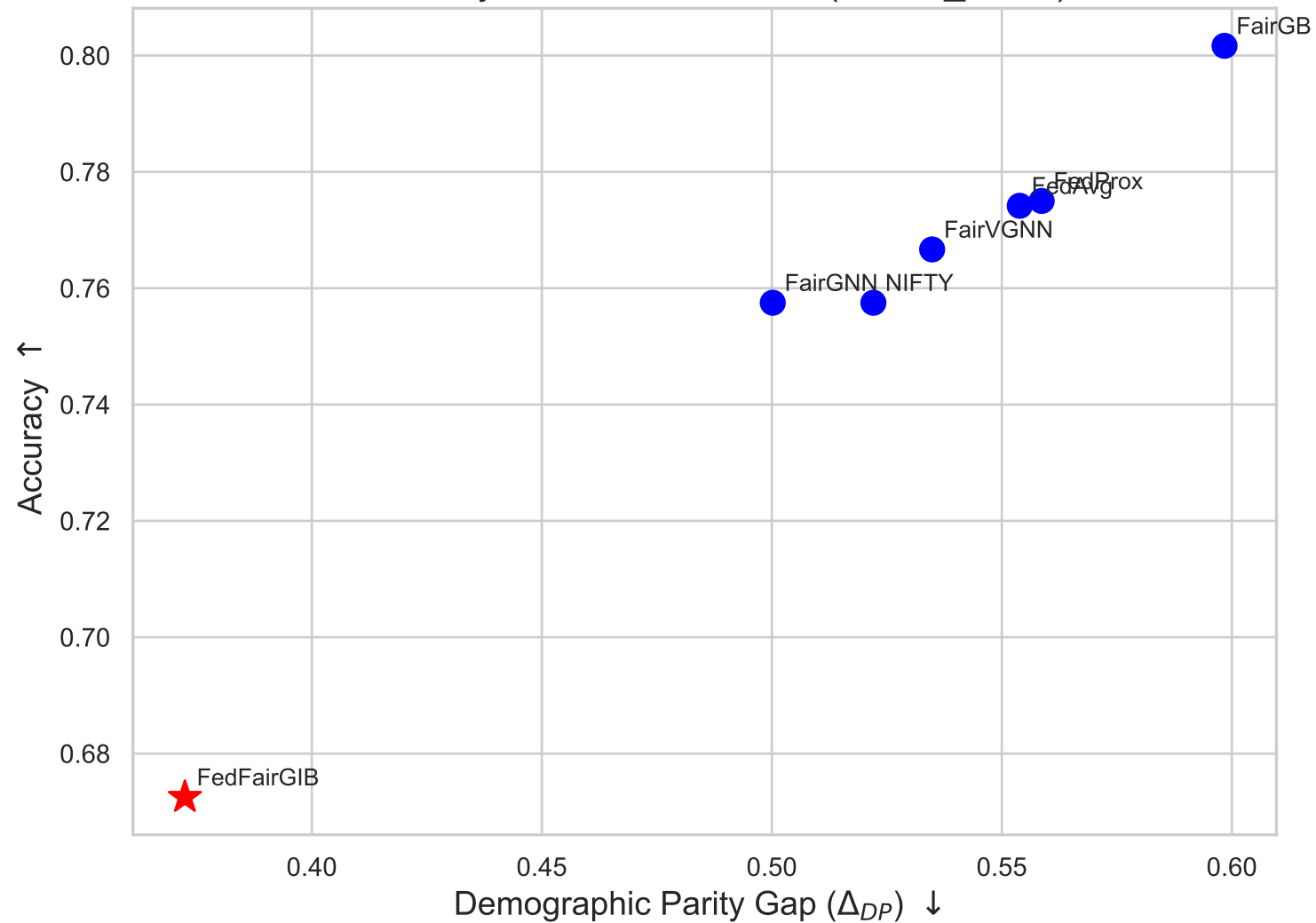
Accuracy-Fairness Trade-off (Pokec_n, IID)
