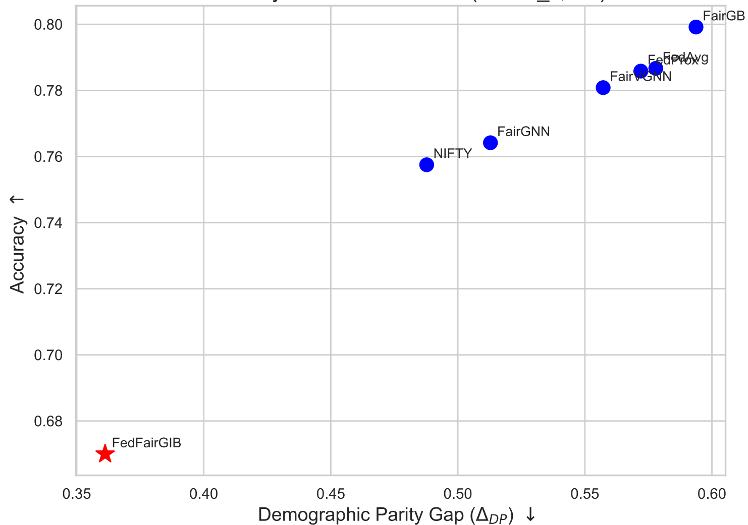
Accuracy-Fairness Trade-off (Pokec_z, IID)
