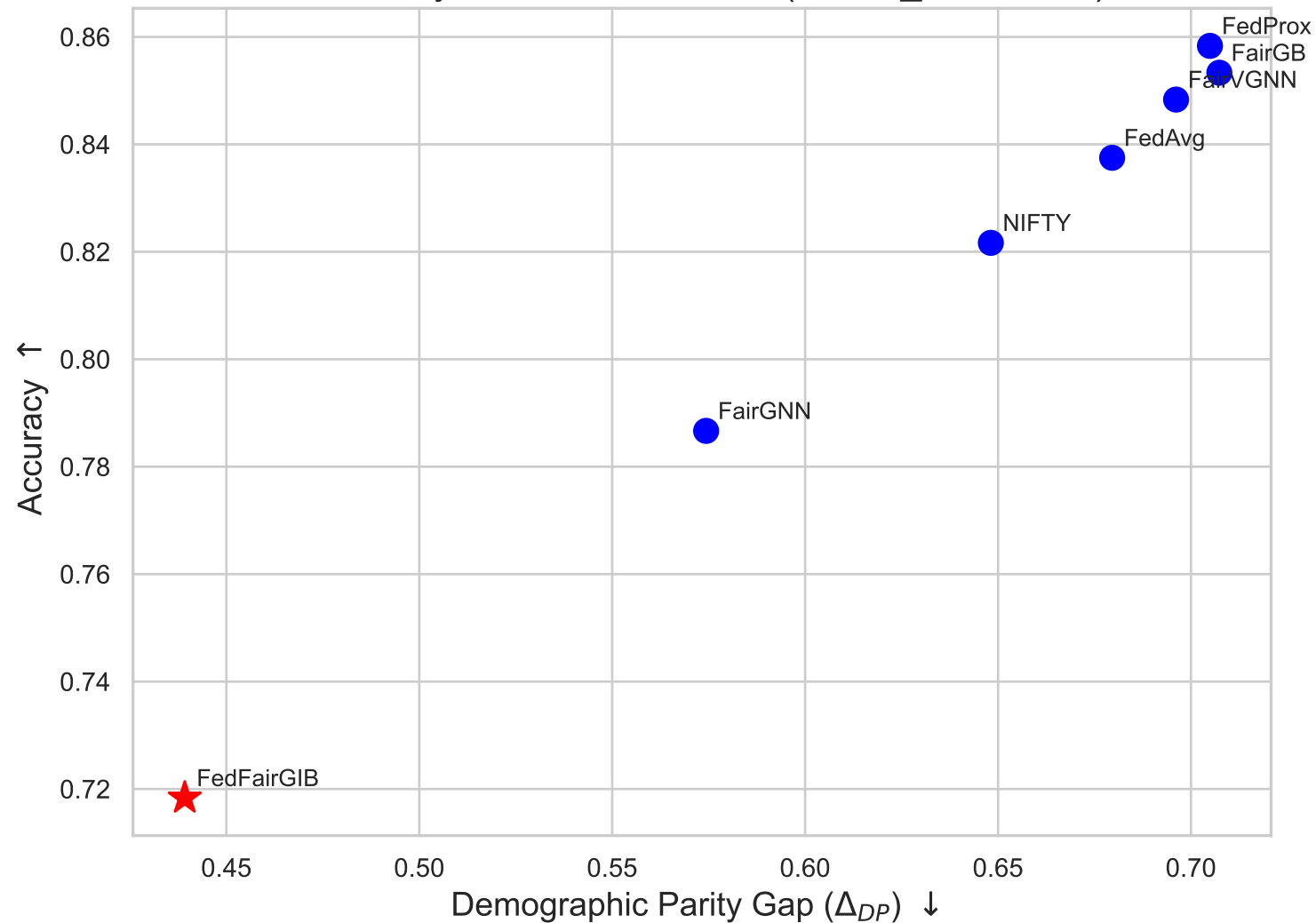
Accuracy-Fairness Trade-off (Pokec_z, NONIID)
