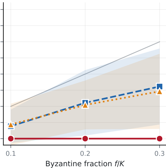
Fairness poisoning
