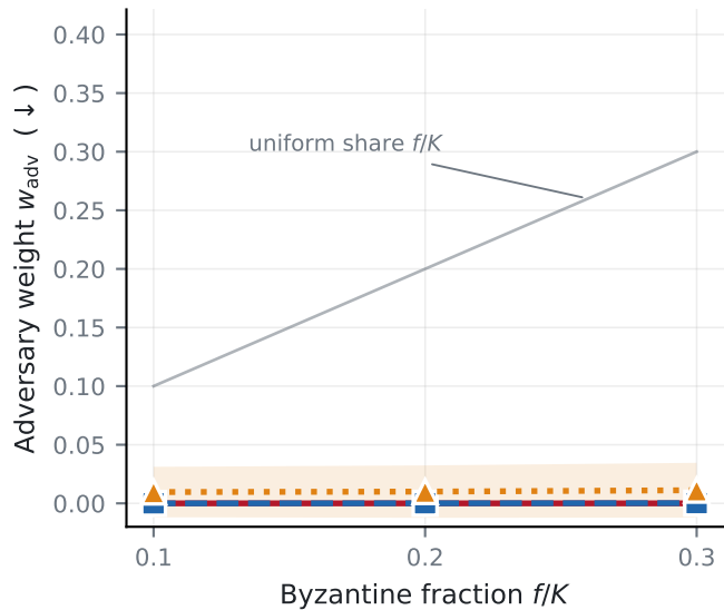
Sign-flip
