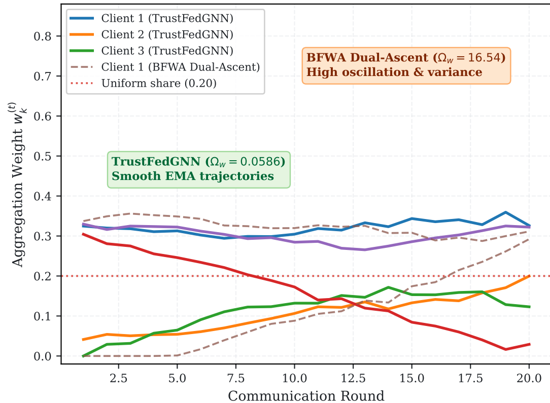
(b) Weight Trajectory Dispersion \Omega_w Across Rounds
