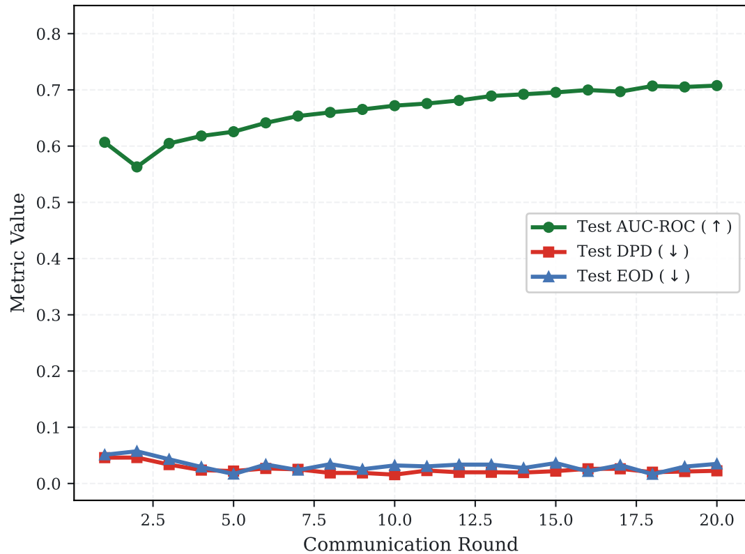
(a) Training Convergence Dynamics (Bail Recidivism)
