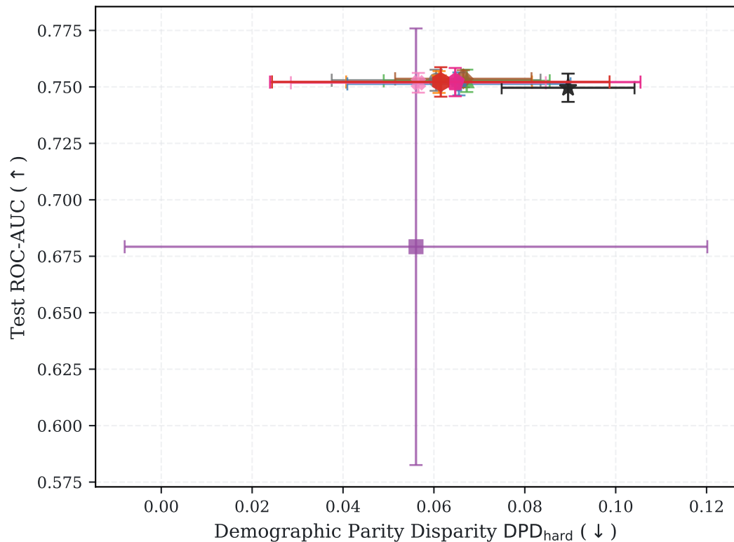
Pareto Frontier: Credit Default ( N = 30,000 )
