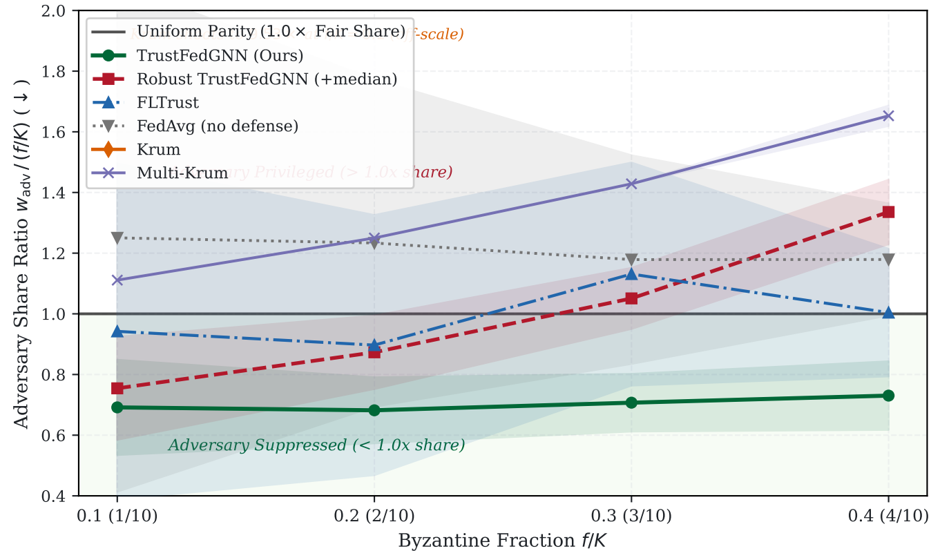
Adversarial Share Ratio under Stealth Poisoning: The Shielding Paradox
