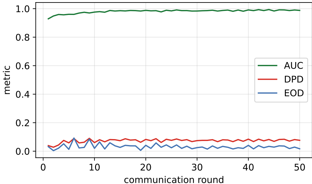
TrustFedGNN convergence (Bail)
