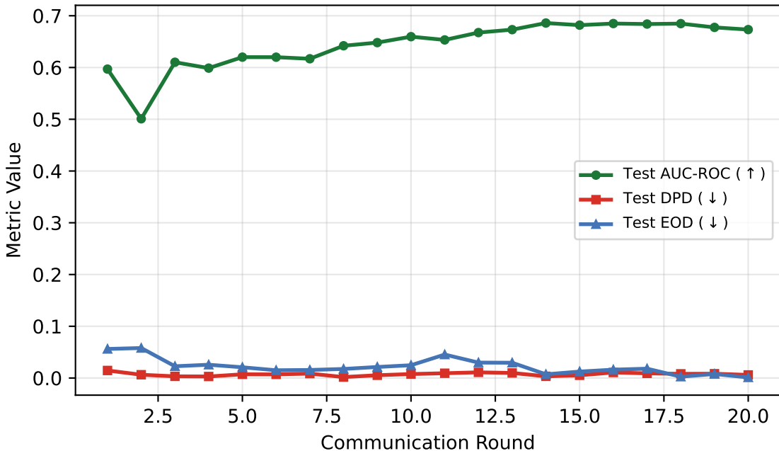
TrustFedGNN Convergence Dynamics (Bail Recidivism)
