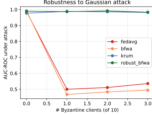
Fig. 5: AUC under Gaussian attack versus number of Byzantine clients (of 10). Robust aggregation retains utility as corruption grows.
