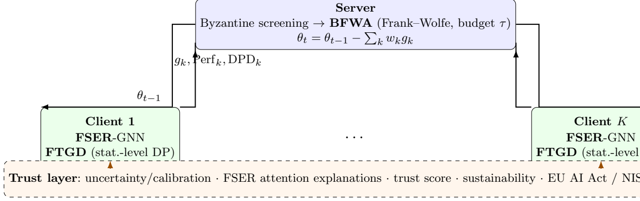
Fig. 1: TrustFedGNN architecture. Three interventions act at complementary control points—FSER inside client message passing, FTGD at the local gradient, and BFWA (with Byzantine screening) at server aggregation—while a trust layer instruments the whole system for audit. Only model weights are transmitted, so fairness and privacy add no communication overhead.
