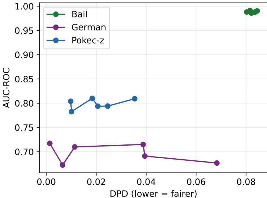
Fairness--utility trade-off (varying \lambda )
