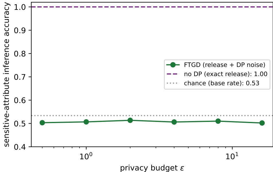
Attribute-inference attack on the released statistic (Bail)
