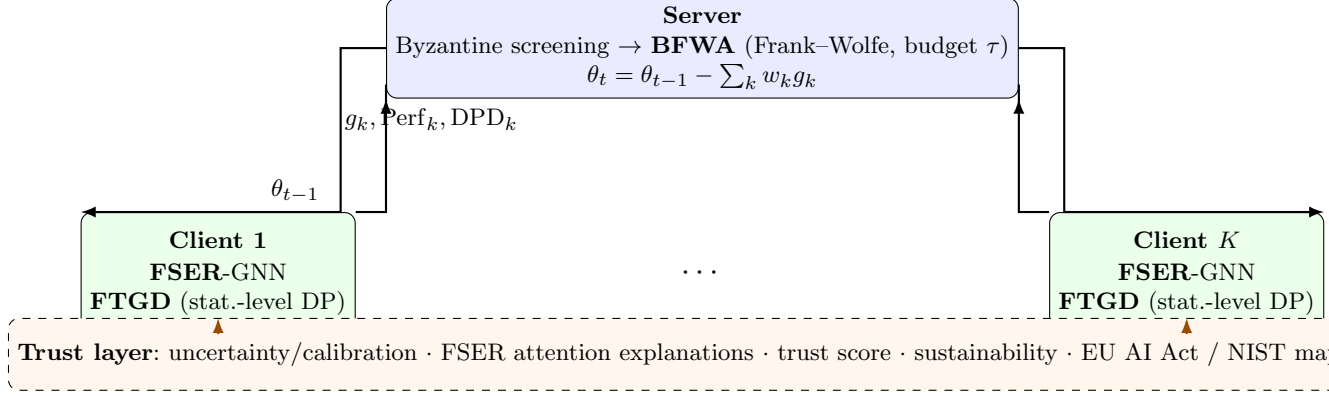
Fig. 1: TrustFedGNN architecture. Three interventions act at complementary control points—FSER inside client message passing, FTGD at the local gradient, and BFWA (with Byzantine screening) at server aggregation—while a trust layer instruments the whole system for audit. Only model weights are transmitted, so fairness and privacy add no communication overhead.
