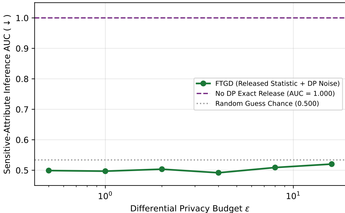
Attribute Inference Defense on Released Statistic (Bail)
