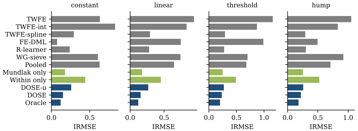
Figure C.2: IRMSE of the estimated effect function by design (stylised design, 100 replications). DOSE denotes Panel-DOSE and DOSE-u its unpenalised version; green bars are ablations; Oracle is the infeasible latent-information benchmark.
