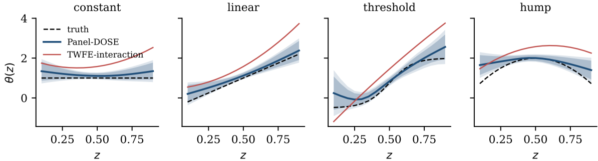
Figure C.3: One simulated sample per design. Dashed black: true \theta(z) ; blue: Panel-DOSE with 95% pointwise (dark) and simultaneous (light) bands; red: TWFE with quadratic interaction.
