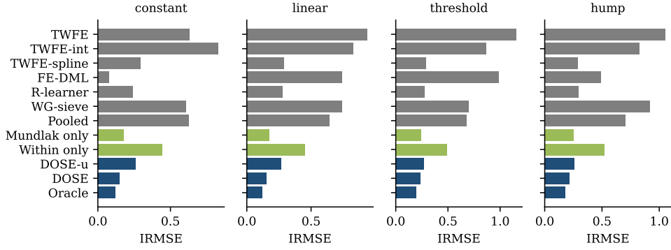
Fig. 1 IRMSE of the estimated effect function by design (stylised design, 100 replications). DOSE denotes Panel-DOSE and DOSE-u its unpenalised version; green bars are ablations; Oracle is the infeasible latent-information benchmark.
