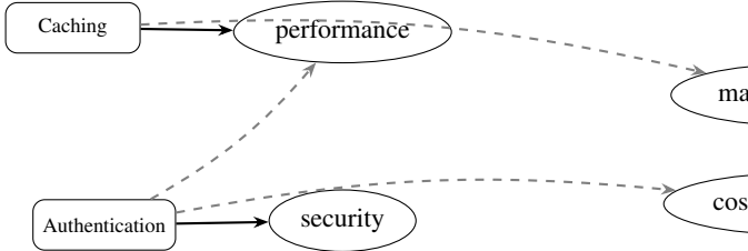
Fig. 2. Excerpt of knowledge graph G : solid arrows are supports edges, dashed gray arrows are trade-off edges. Only 2 of the catalog's 26 tactics and 4 of its 5 quality attributes are shown for legibility.
