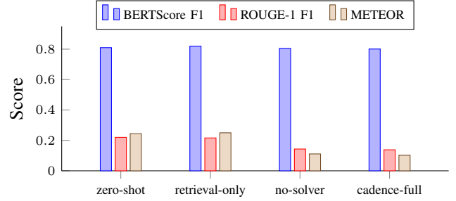
Fig. 3. Pilot run (Table V): BERTScore F1 stays flat across all four systems while ROUGE-1 and METEOR drop sharply for the two deliberation-based systems ( no-solver = multiagent_no_solver ) — the length/register mismatch this section discusses, not a quality gap.
