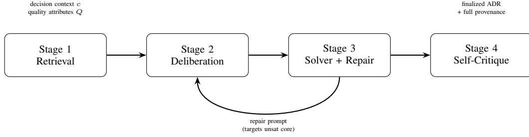
Fig. 1. The CADENCE pipeline. Each stage consumes the previous stage’s output; Stage 3’s repair loop feeds a targeted prompt, derived from the solver’s unsatisfiable core, back into Stage 2’s synthesizer, iterating to a fixed cap before Stage 4 finalizes the decision.
