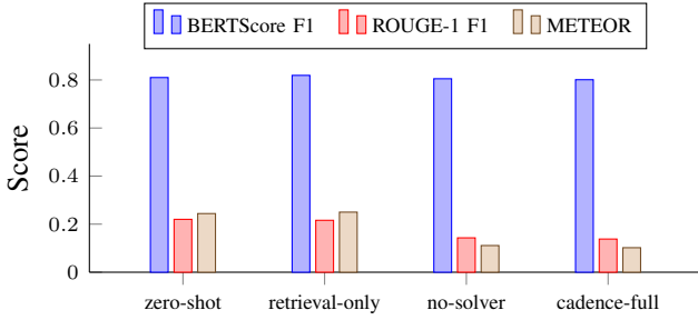
Fig. 3. Pilot run (Table V): BERTScore F1 stays flat across all four systems while ROUGE-1 and METEOR drop sharply for the two deliberation-based systems (no-solver = multiagent_no_solver) — the length/register mismatch this section discusses, not a quality gap.
