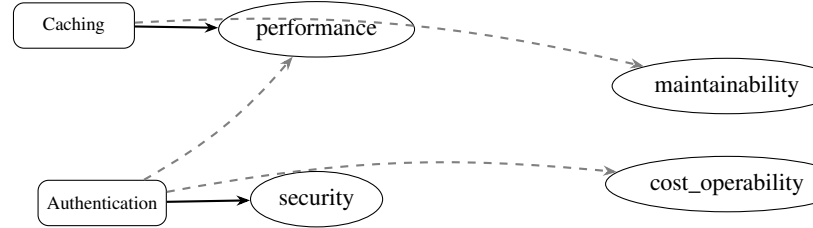
Fig. 2. Excerpt of knowledge graph G : solid arrows are supports edges, dashed gray arrows are trade-off edges. Only 2 of the catalog’s 26 tactics and 4 of its 5 quality attributes are shown for legibility.
