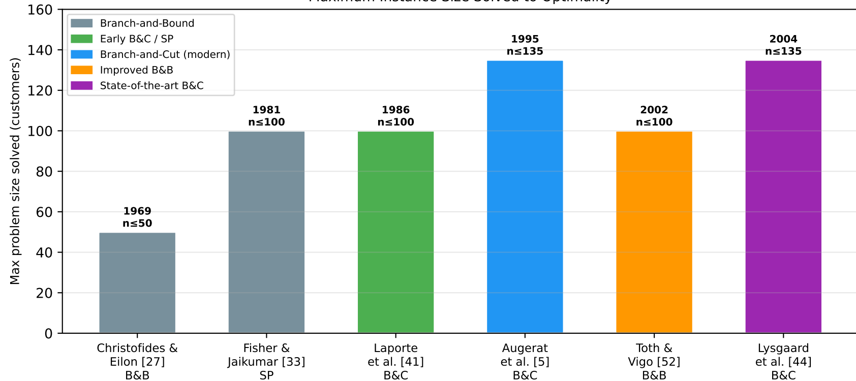
Progress of Exact CVRP Algorithms: Maximum Instance Size Solved to Optimality
