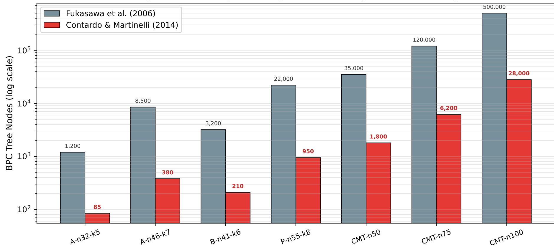
Number of BPC Tree Nodes: 2006 vs. 2014 Algorithms SRCs + ng-routes + strong branching reduce nodes by 1-2 orders of magnitude
