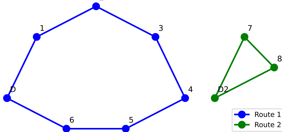
Before Or-opt: node 3 in Route 1
