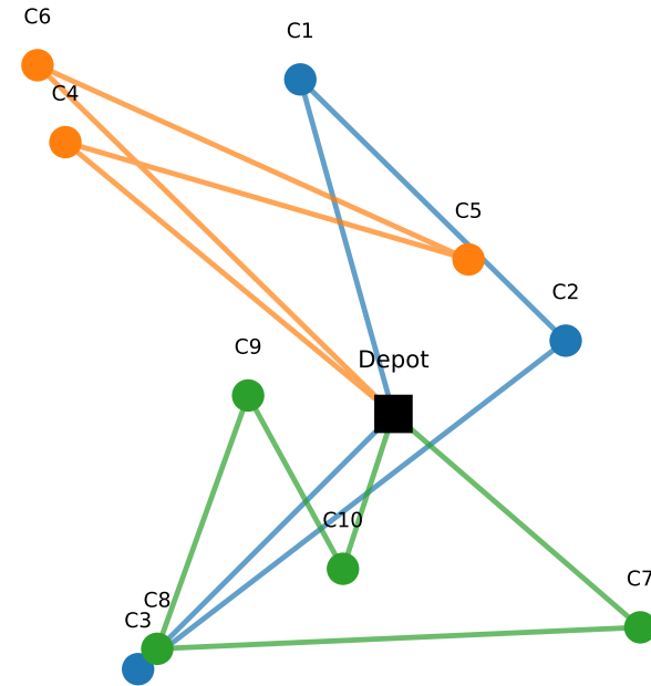
Repair Phase (re-insert removed customers optimally)
