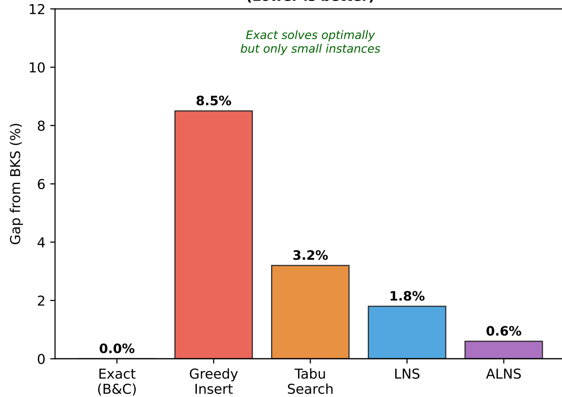
Average Gap from Best Known Solution (%) (Lower is better)
