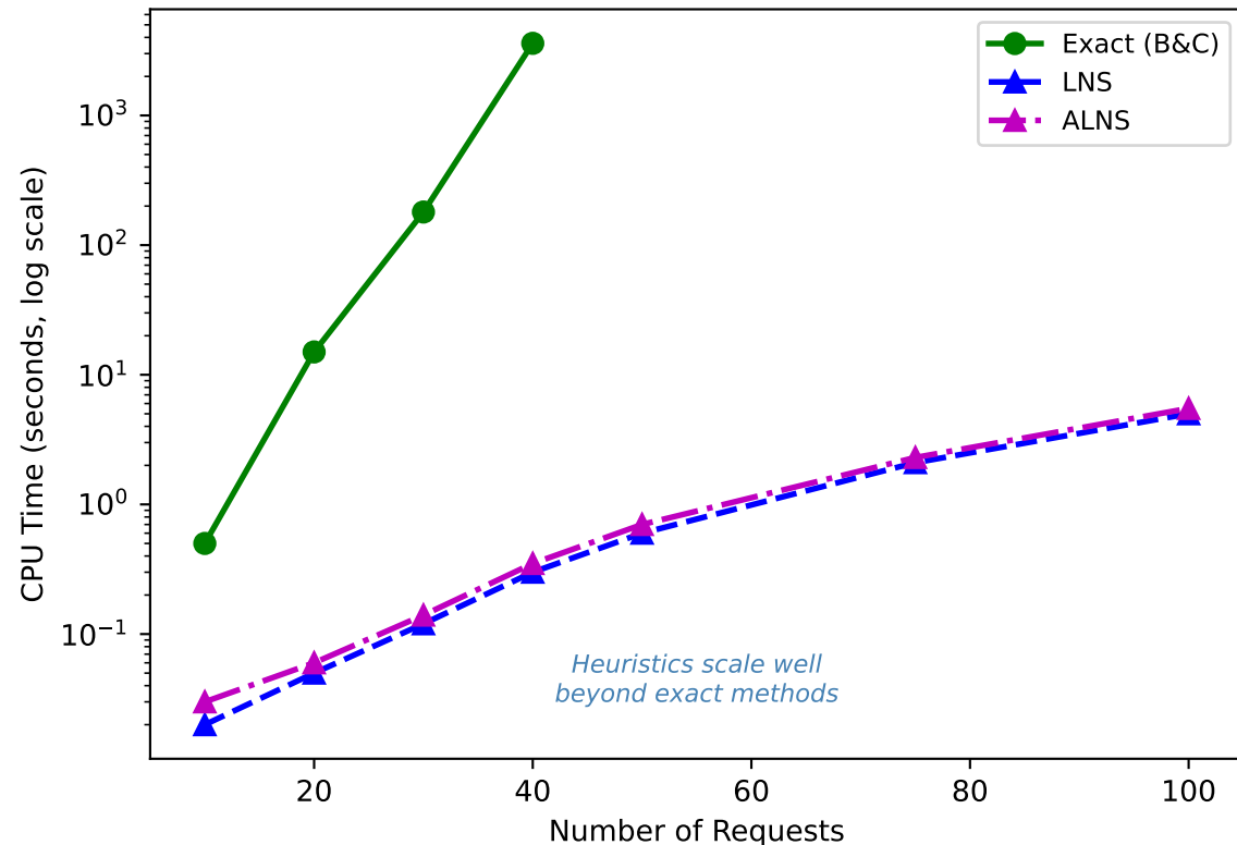
CPU Time vs Instance Size (Log scale)
